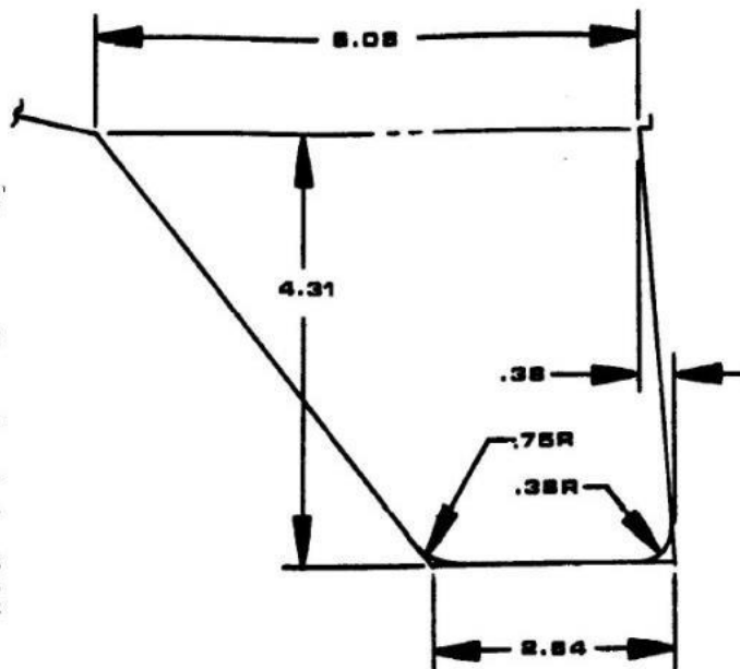
GEAR CASE SKEG HALF SIZE
