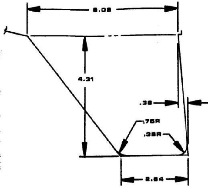
GEAR CASE SKEG HALF SIZE
